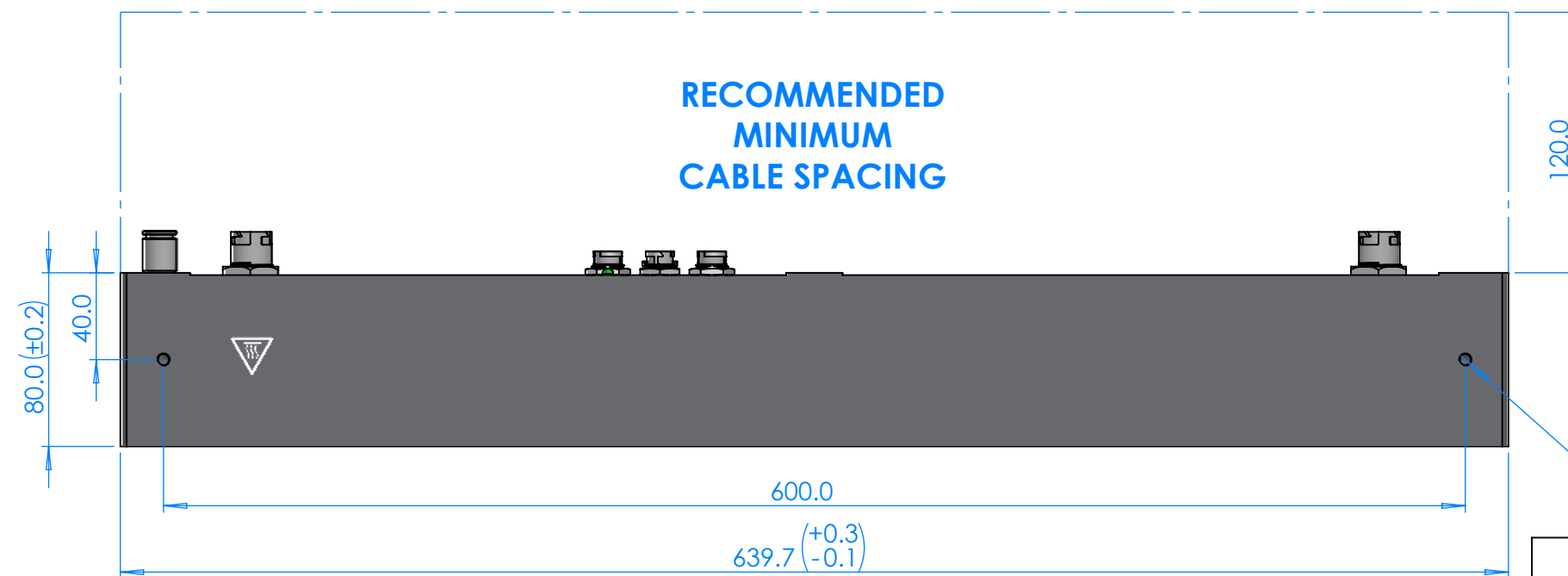
SIDE VIEW
